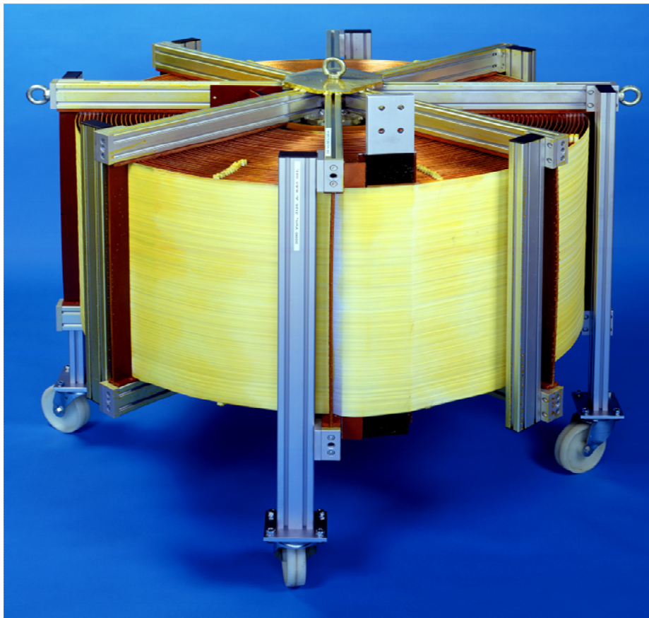
Air-cored reactor 3125 A 0.63 mH
